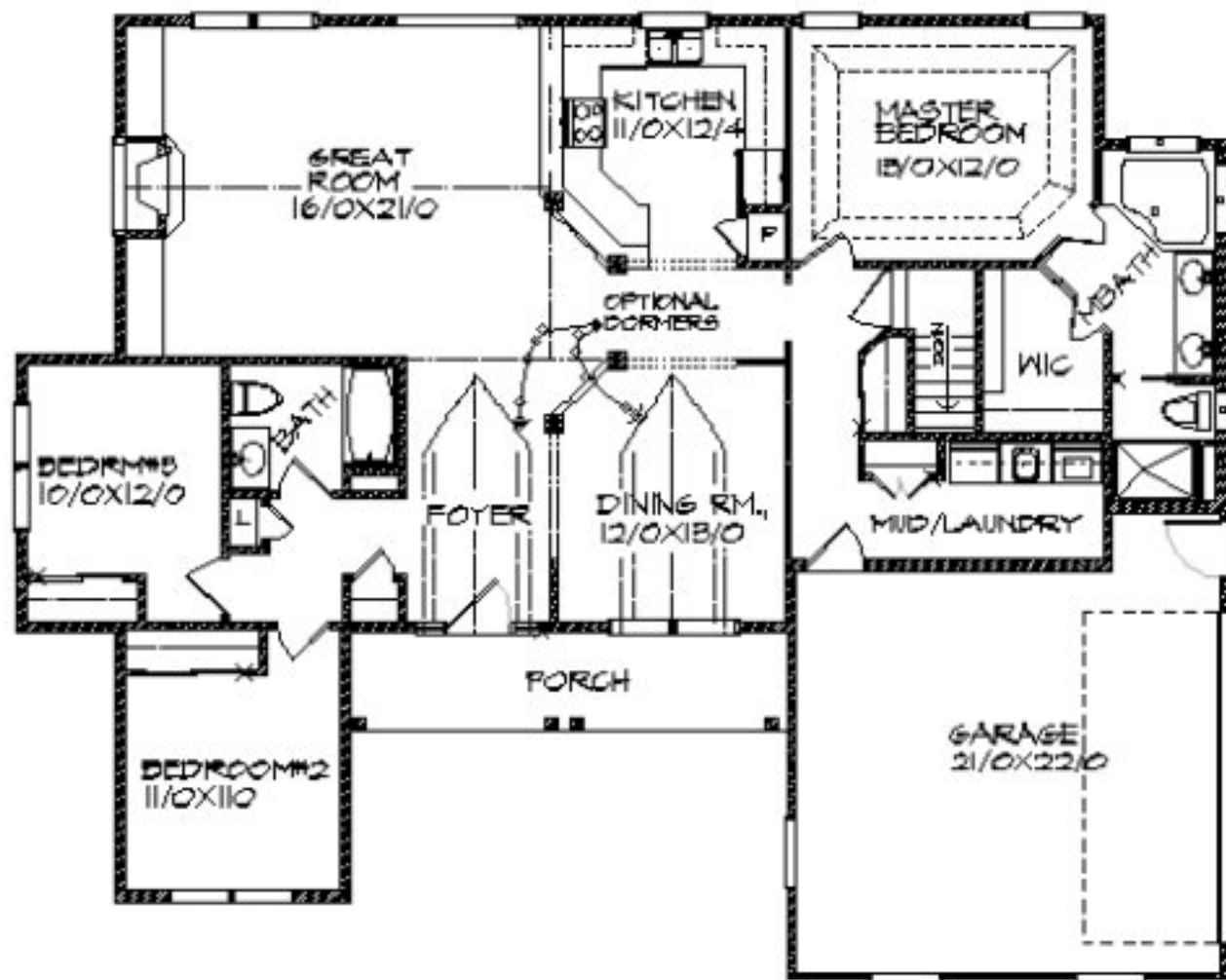
FLOOR PLAN 59/0X47/0
