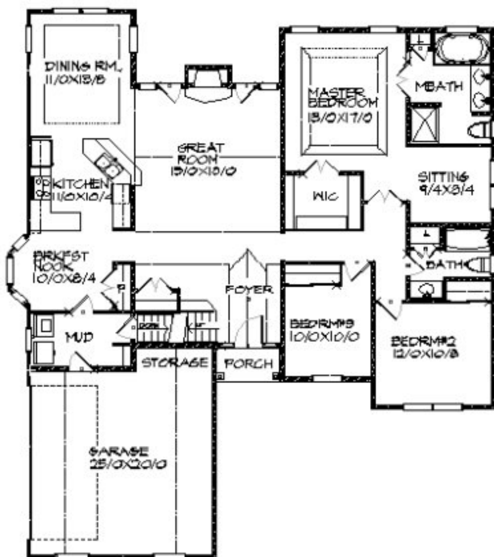
FLOOR PLAN 64X60
