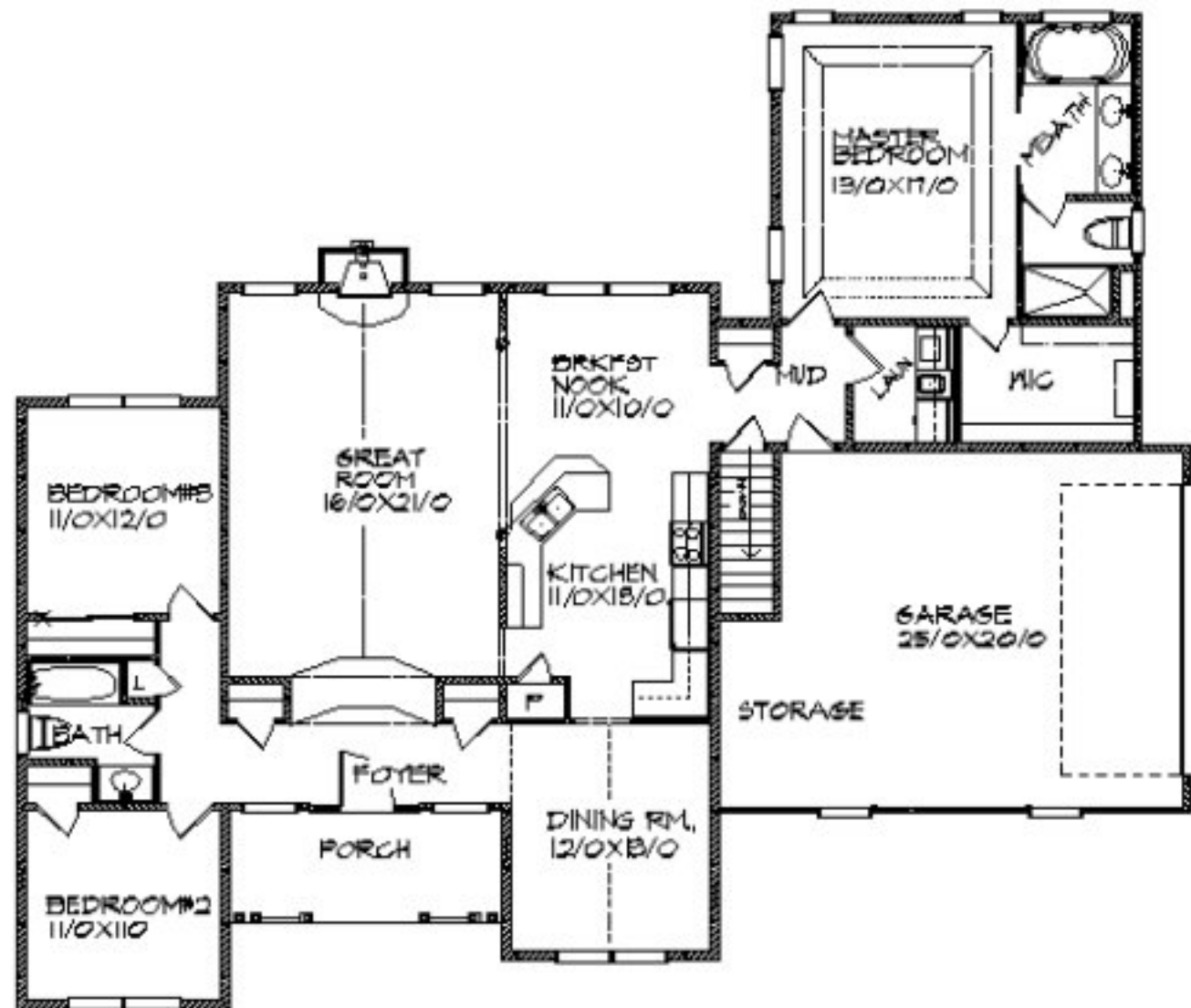
FLOOR PLAN 64X58
