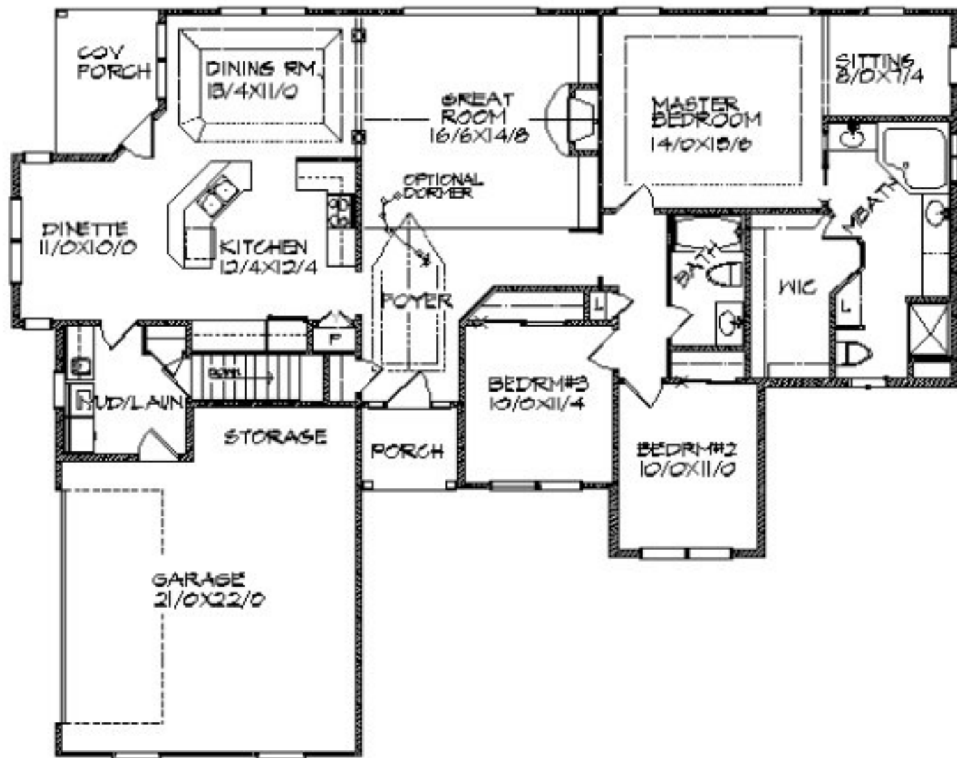
FLOOR PLAN 65/0x52/0
